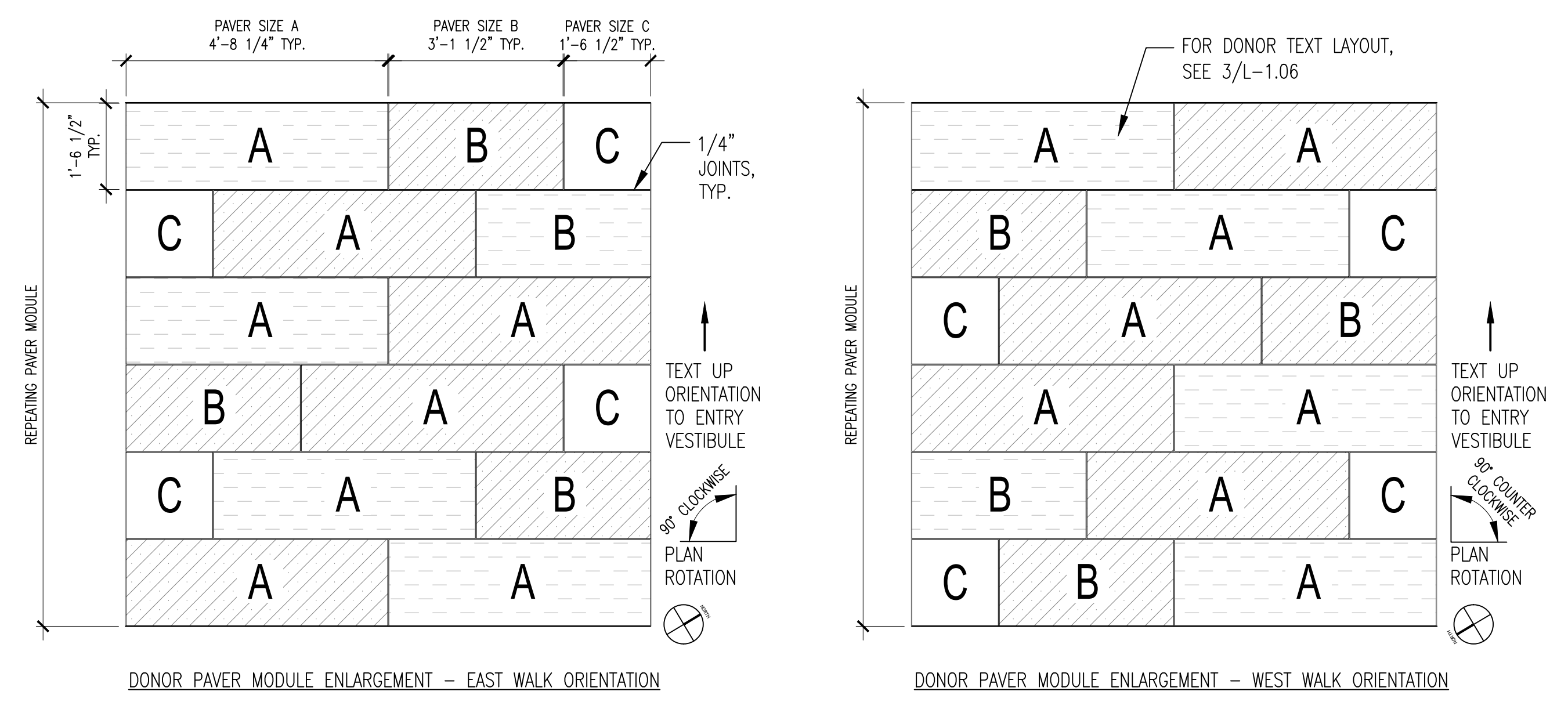
2 DONOR PAVER MODULE ENLARGEMENT L1.06 SCALE: 1/2" = 1'-0"
