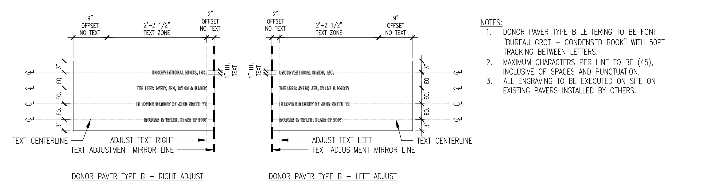
5 DONOR PAVER TYPE B ENGRAVING LAYOUT L1.06 SCALE: 1" = 1'-0"
